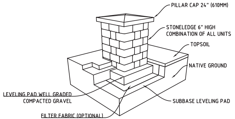
22" STONELEDGE PILLAR DETAIL
