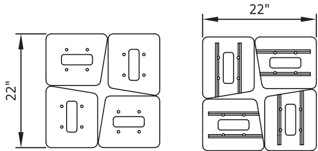
22" STONELEDGE PILLAR DETAIL
