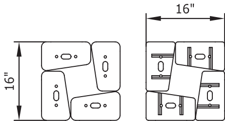
16" STONELEDGE PILLAR DETAIL
