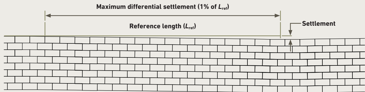
Differential settlement
