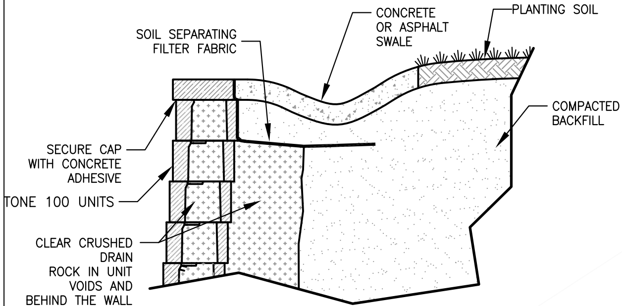
CONCRETE OR ASPHALT SWALE SECTION
