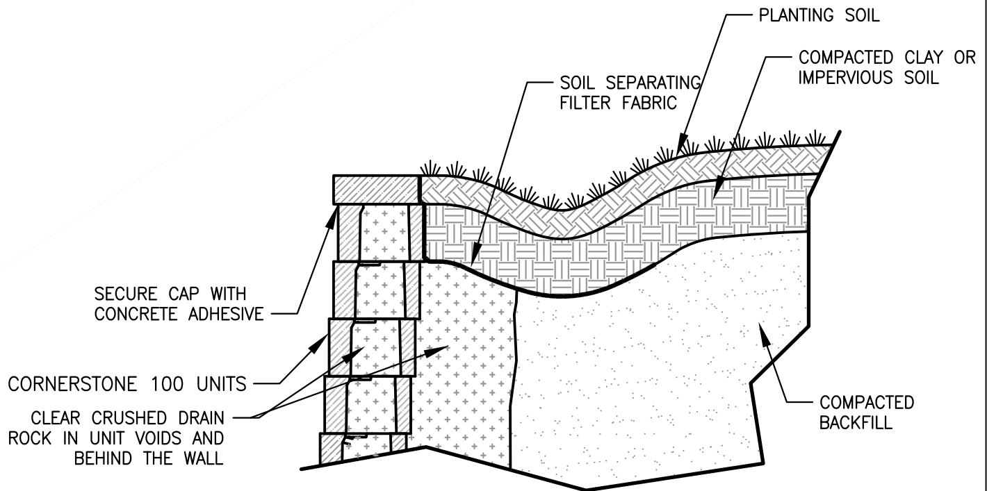
COMPACTED CLAY OR IMPERVIOUS SOIL SWALE SECTION
